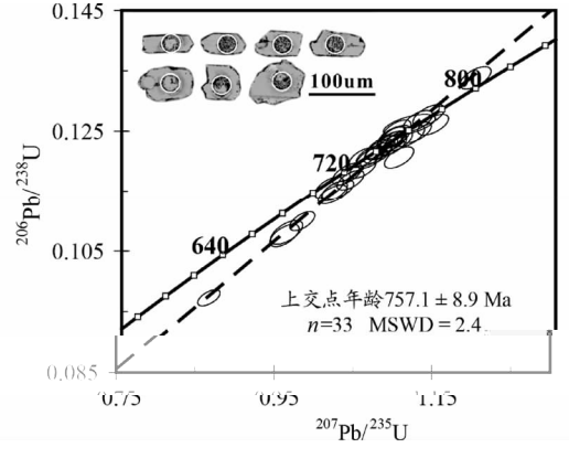
5 AKS01 BSE U-Pb
